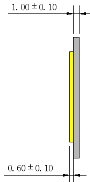
Fig.1-2 Side view 侧面视图
