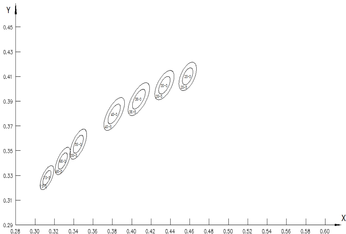
Fig 1-4 The C.I.E Chromaticity Diagram CIE色度图
